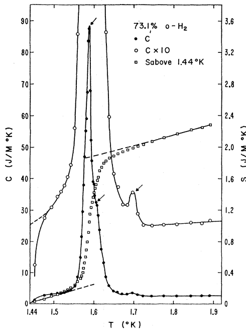
FIG. 4. The λ anomaly at zero pressure and 73.1% orthohydrogen. The arrows indicate distinguishable peaks.
