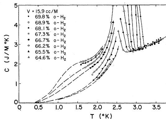
FIG. 12. The heat capacity in the vicinity of the \lambda anomaly at 15.9 cc/mole at several concentrations.
