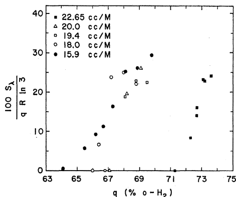
FIG. 7. The relative contribution (at several molar volumes) of the \lambda anomaly entropy as a function of concentration.
