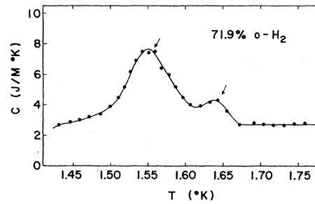
FIG. 5. The λ anomaly at zero pressure and 71.9% orthohydrogen. The arrows indicate distinguishable peaks.
