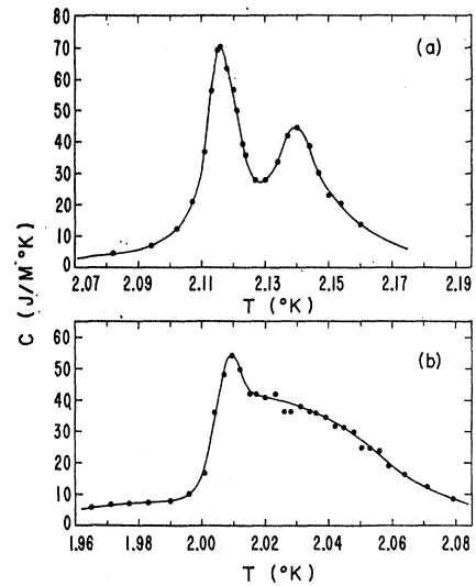
FIG. 11. Typical shapes of the \lambda anomaly at small molar volumes. (a) and (b) were measured in cells I and II, respectively, under similar conditions.
