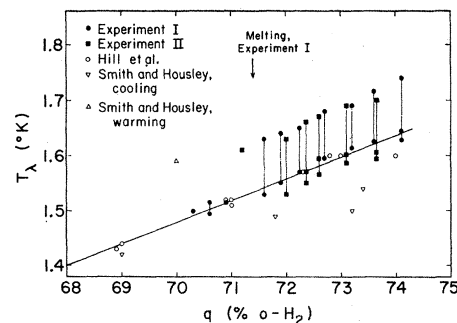
FIG. 6. The λ temperature as a function of concentration at zero pressure. The points connected vertically are separate peaks observed during the same heating. The arrow labeled melting experiment I indicates the concentration at which the sample was melted and recooled.
